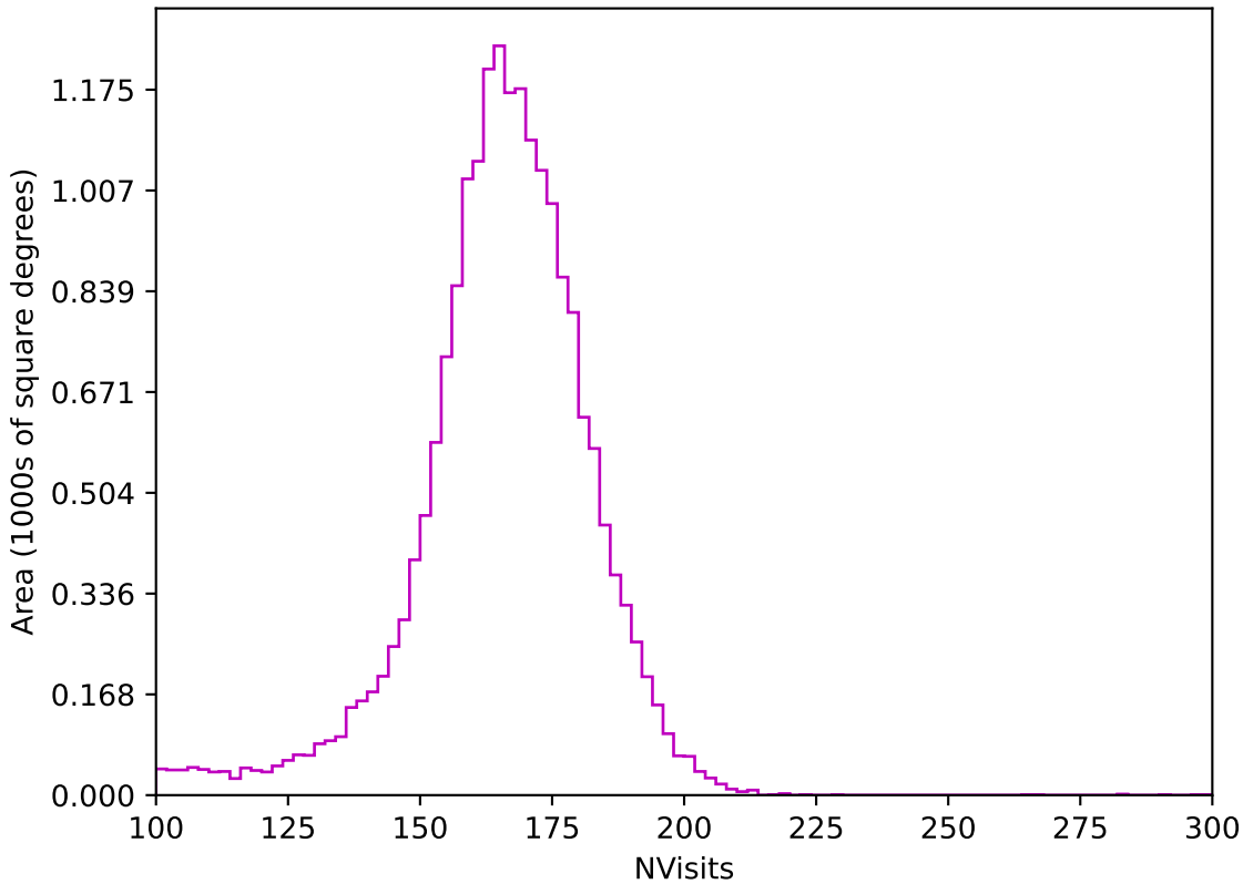
too_elab_r128_d2_griz_v3.4_10yrs All sky z band: NVisits
