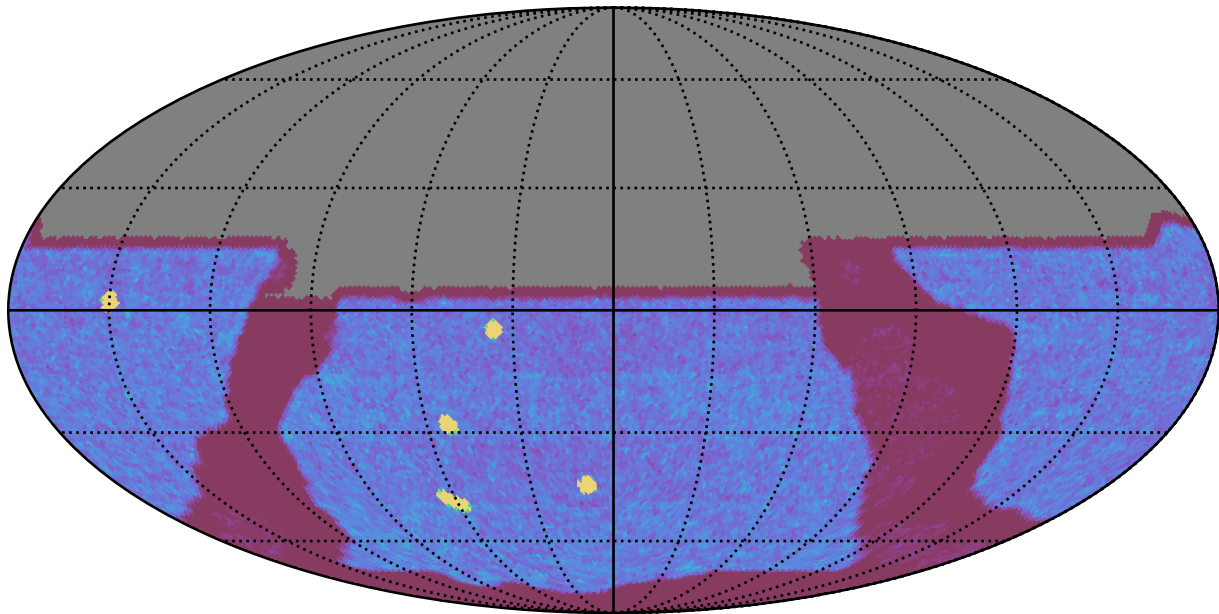
too_elab_r128_d2_griz_v3.4_10yrs All sky y band: NVisits
