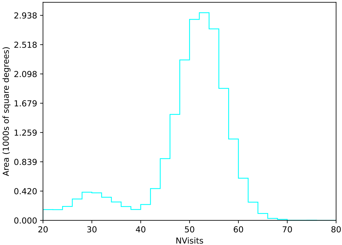
too_elab_r128_d2_griz_v3.4_10yrs All sky u band: NVisits
