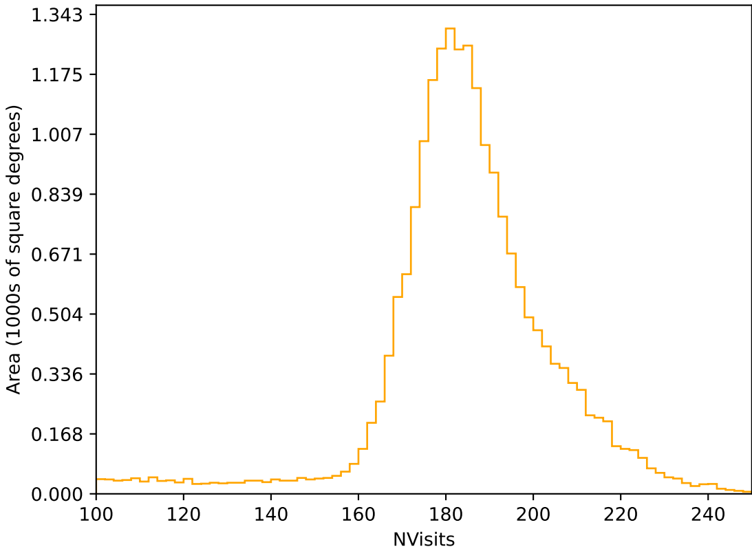
too_elab_r128_d2_griz_v3.4_10yrs All sky r band: NVisits
