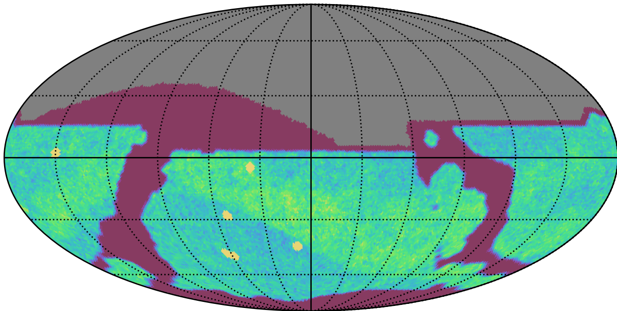
too_elab_r128_d2_griz_v3.4_10yrs All sky i band: NVisits
