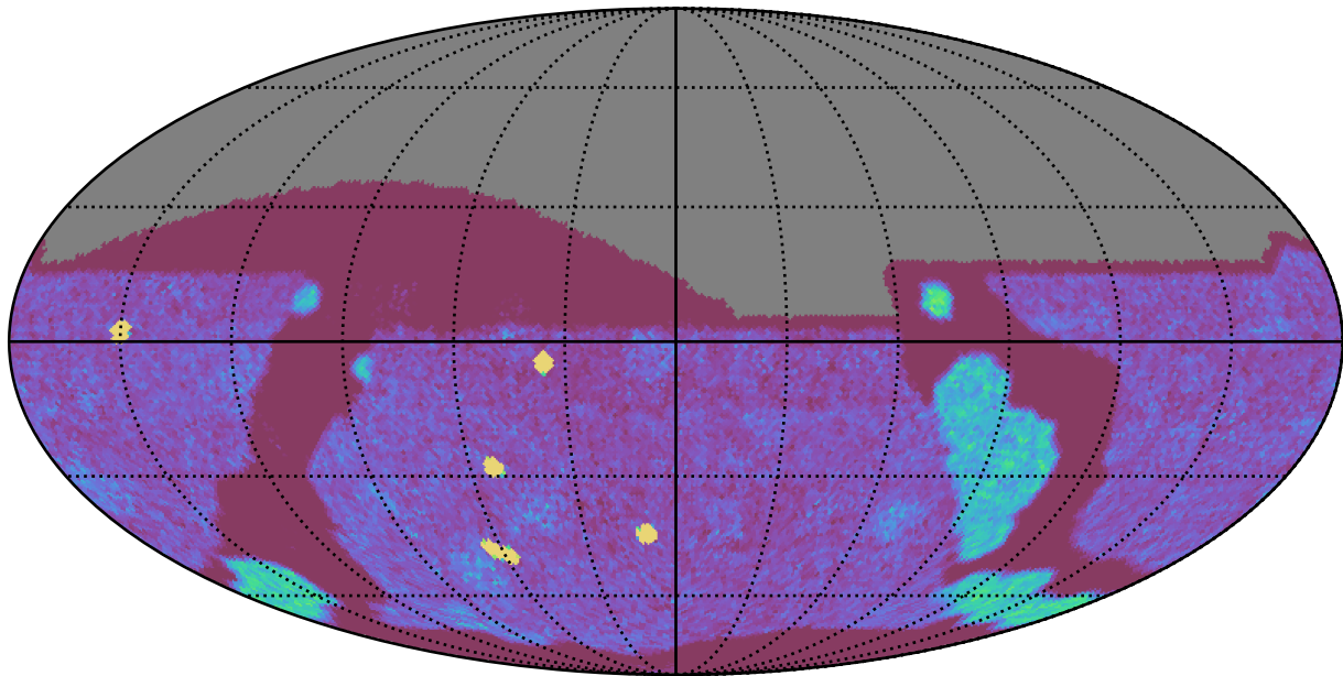
too_elab_r128_d2_griz_v3.4_10yrs All sky g band: NVisits
