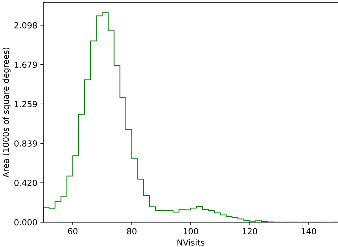
too_elab_r128_d2_griz_v3.4_10yrs All sky g band: NVisits
