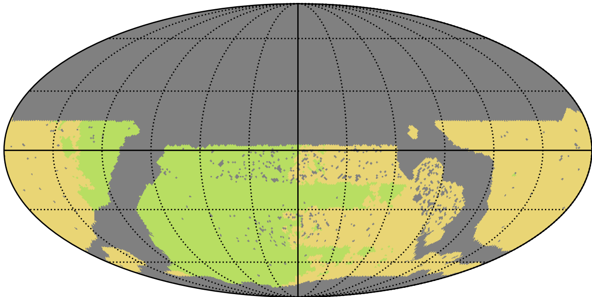
too_elab_r128_d2_griz_v3.4_10yrs WFD all bands: NSeasons
