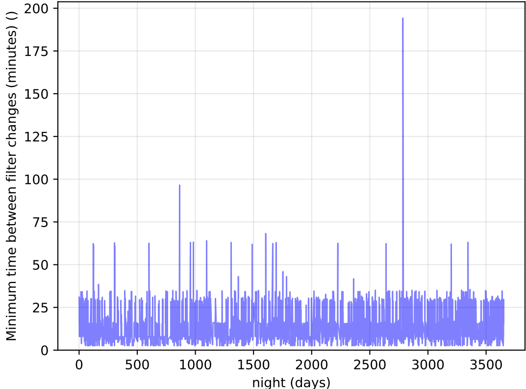
too_elab_r128_d2_griz_v3.4_10yrs Per Night: Minimum time between filter changes (minutes)
