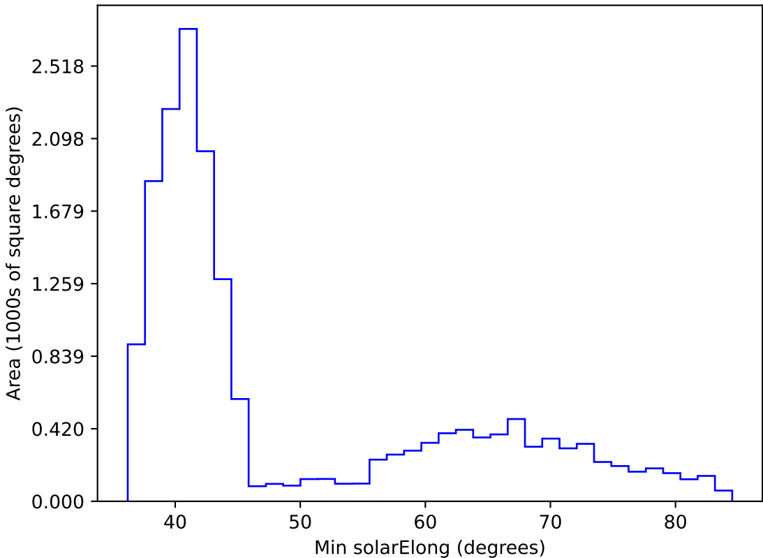
too_elab_r128_d2_griz_v3.4_10yrs WFD z band: Min solarElong
