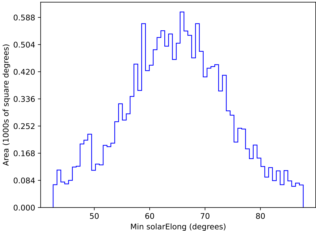
too_elab_r128_d2_griz_v3.4_10yrs WFD y band: Min solarElong
