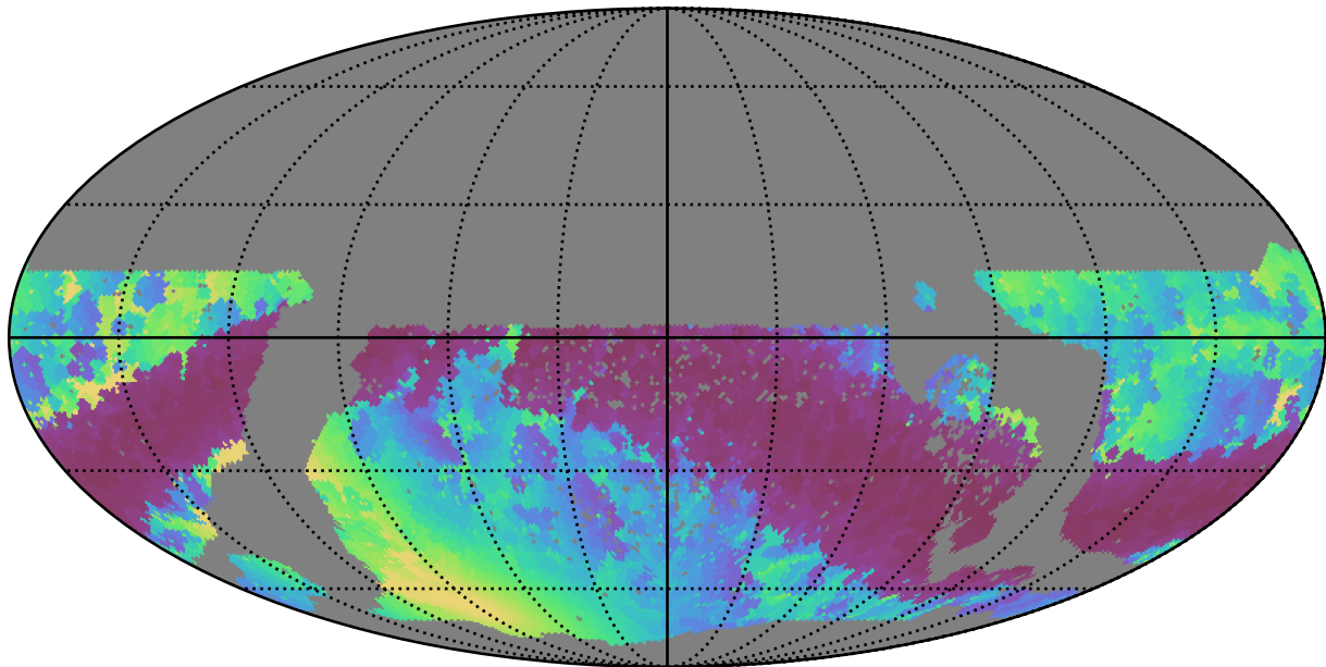
too_elab_r128_d2_griz_v3.4_10yrs WFD r band: Min solarElong
