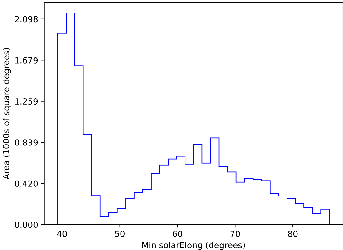
too_elab_r128_d2_griz_v3.4_10yrs WFD r band: Min solarElong
