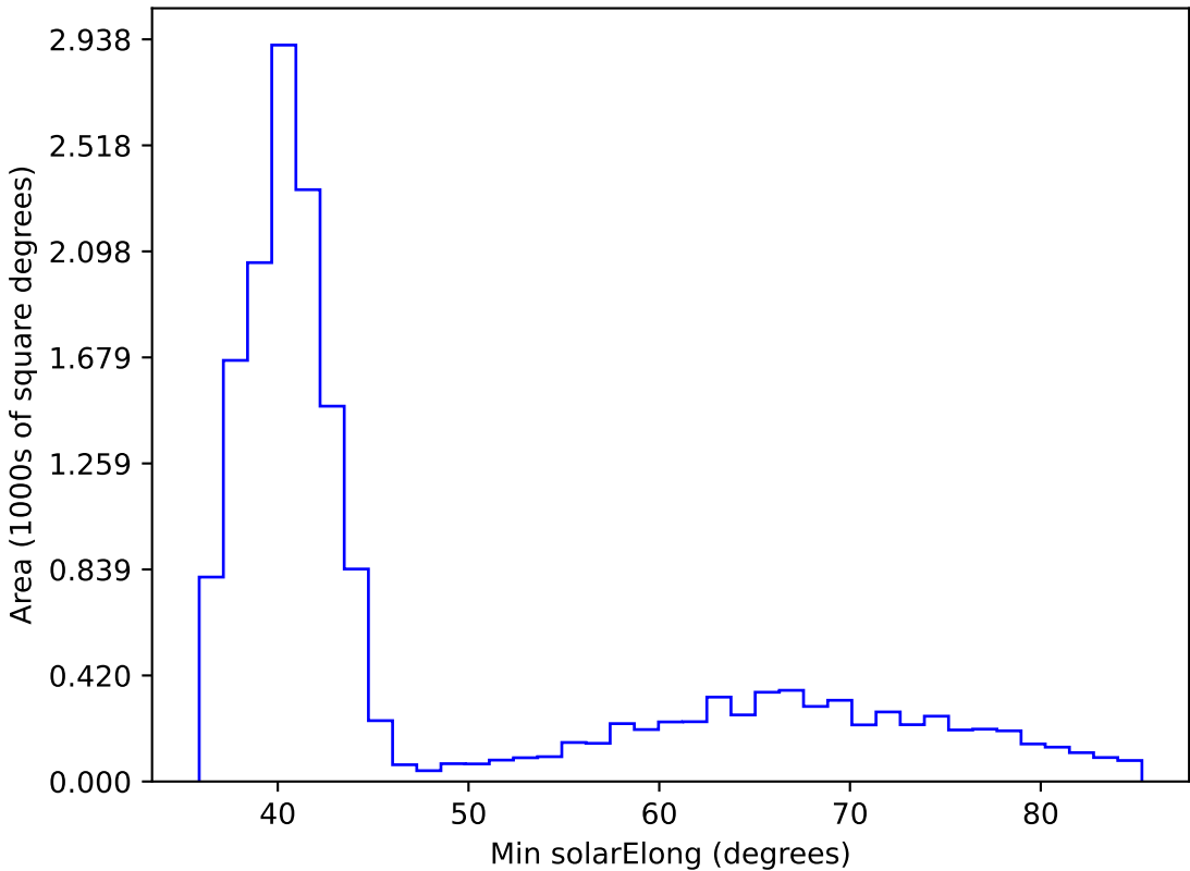
too_elab_r128_d2_griz_v3.4_10yrs WFD i band: Min solarElong
