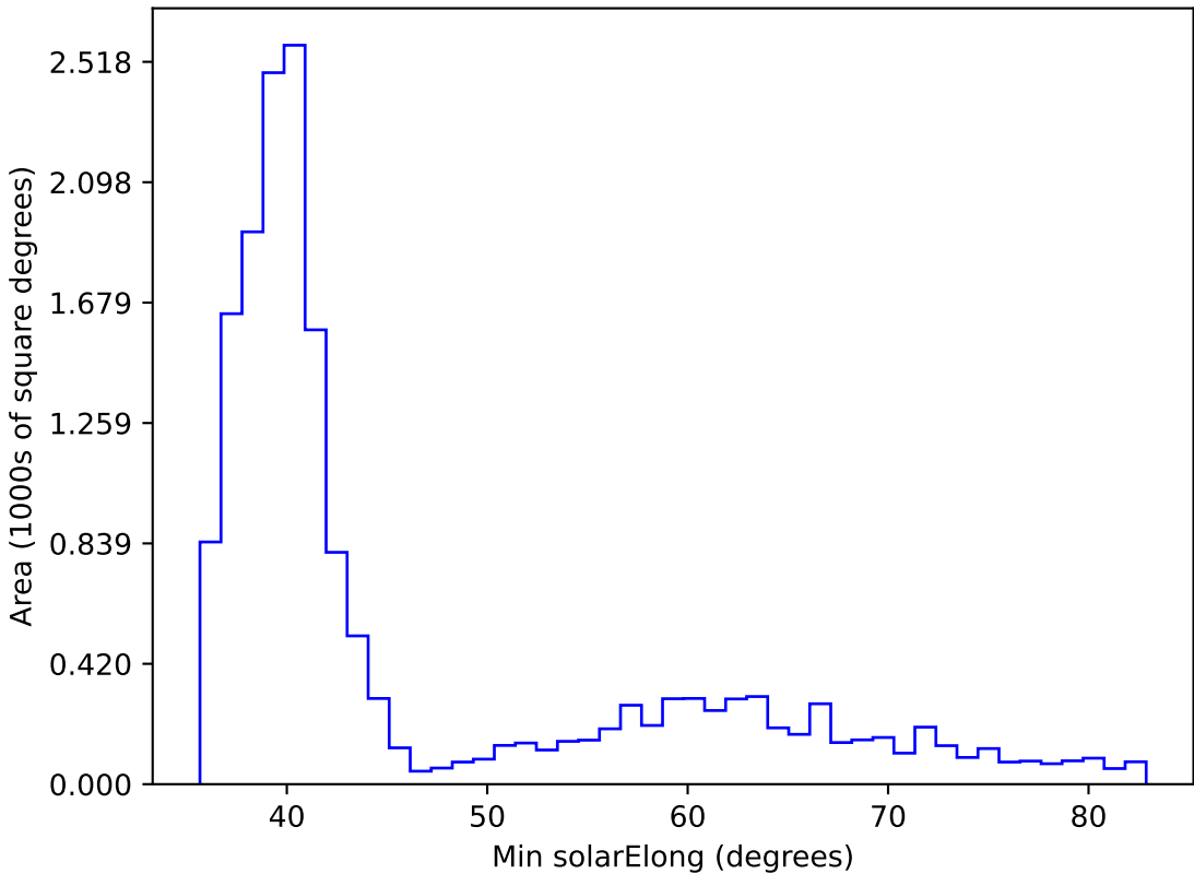
too_elab_r128_d2_griz_v3.4_10yrs WFD all bands: Min solarElong
