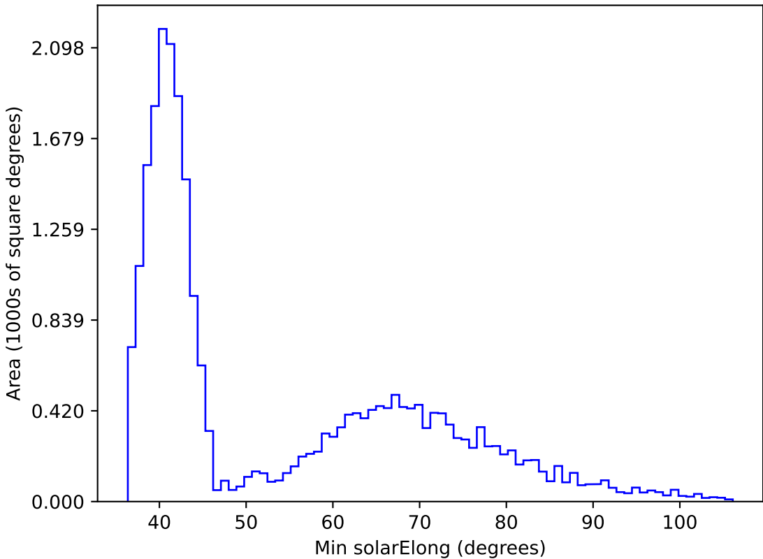
too_elab_r128_d2_griz_v3.4_10yrs All sky z band: Min solarElong
