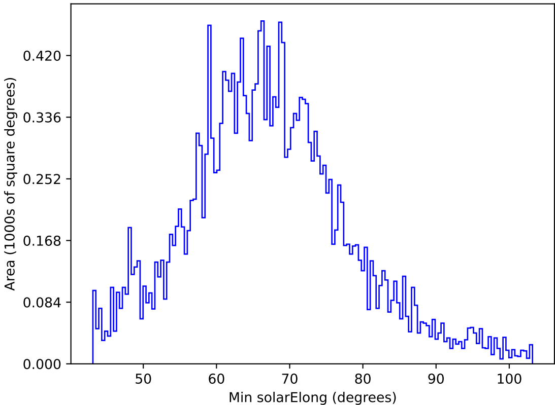
too_elab_r128_d2_griz_v3.4_10yrs All sky y band: Min solarElong
