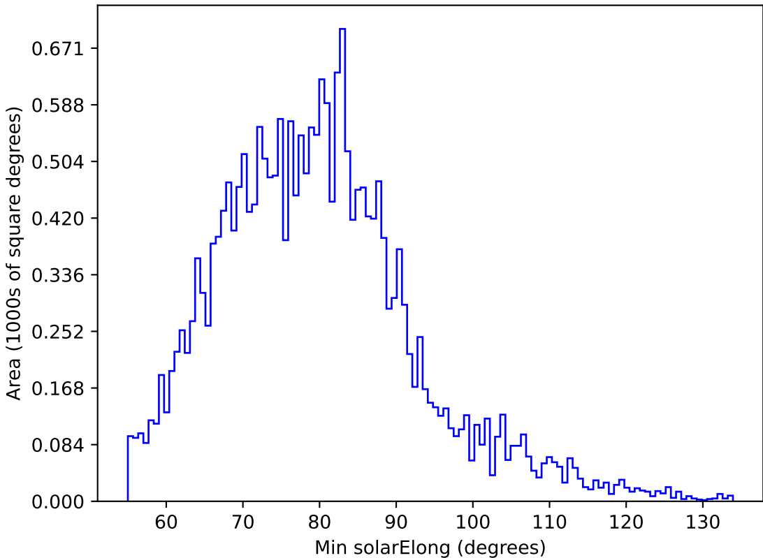
too_elab_r128_d2_griz_v3.4_10yrs All sky u band: Min solarElong
