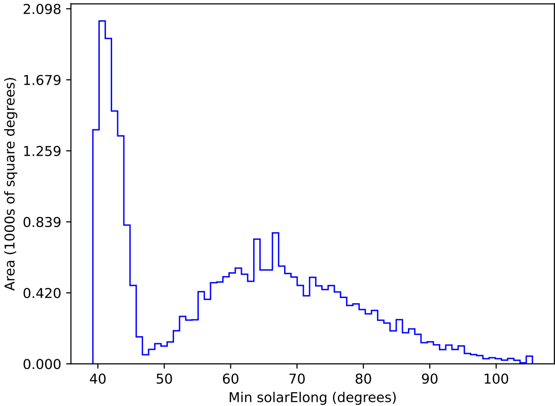
too_elab_r128_d2_griz_v3.4_10yrs All sky r band: Min solarElong
