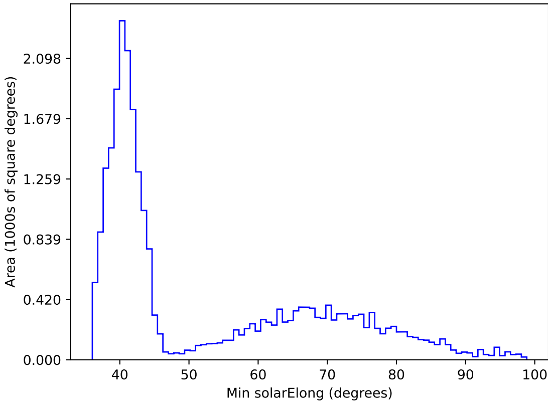
too_elab_r128_d2_griz_v3.4_10yrs All sky i band: Min solarElong
