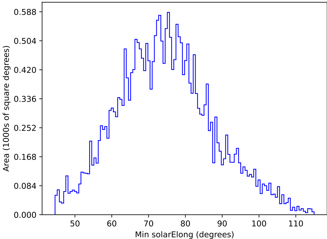
too_elab_r128_d2_griz_v3.4_10yrs All sky g band: Min solarElong
