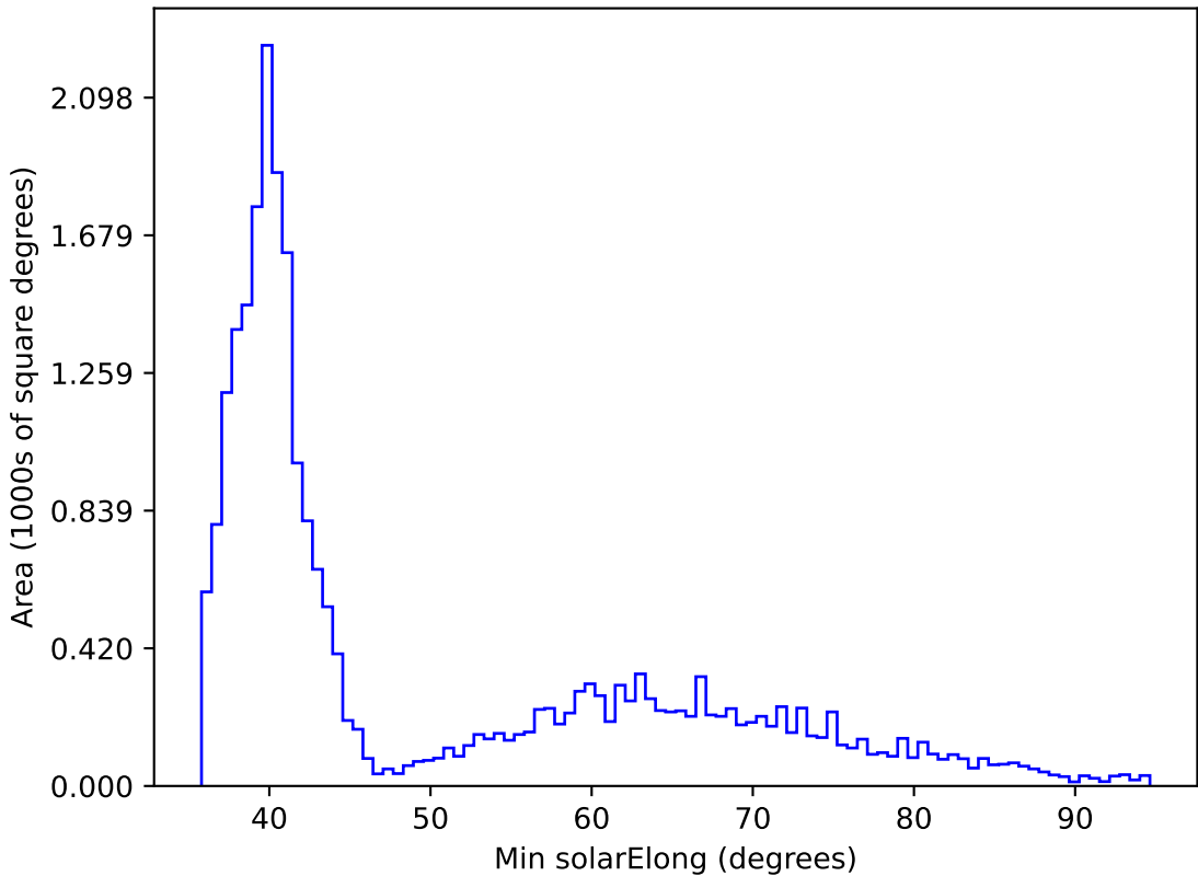
too_elab_r128_d2_griz_v3.4_10yrs All sky all bands: Min solarElong
