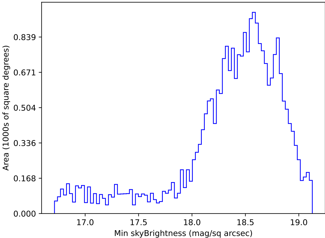
too_elab_r128_d2_griz_v3.4_10yrs Yr 1 z band: Min skyBrightness
