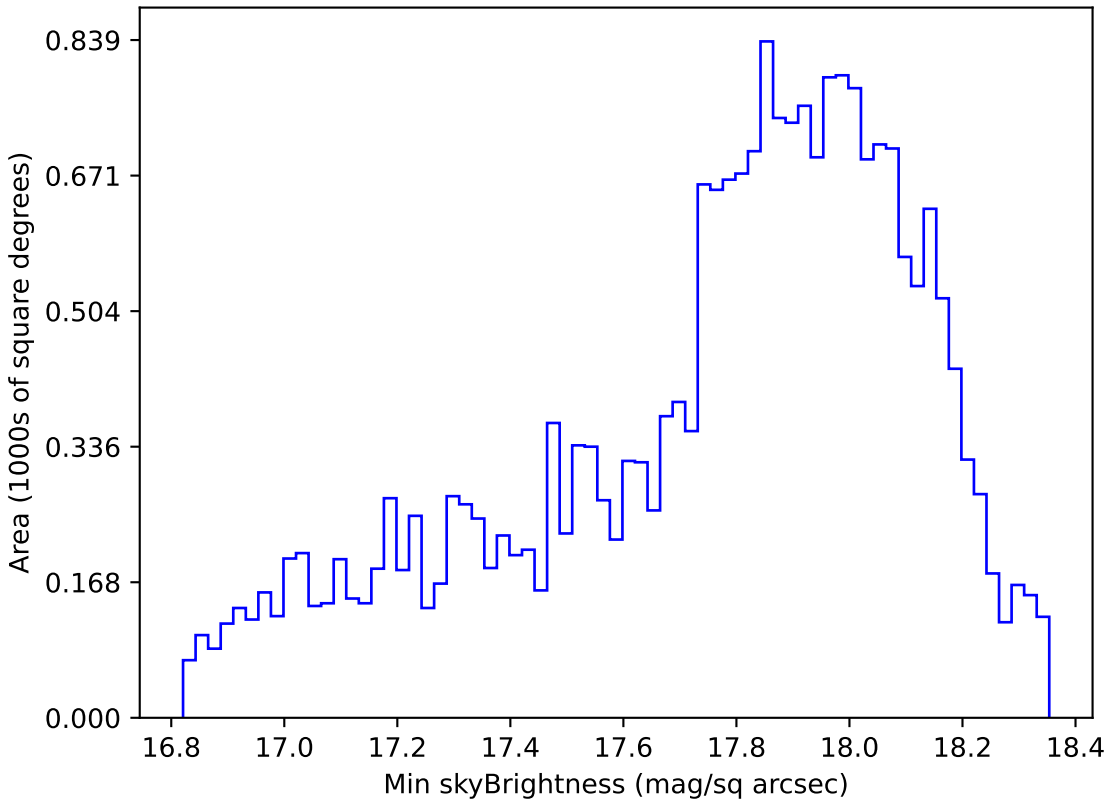
too_elab_r128_d2_griz_v3.4_10yrs Yr 1 y band: Min skyBrightness
