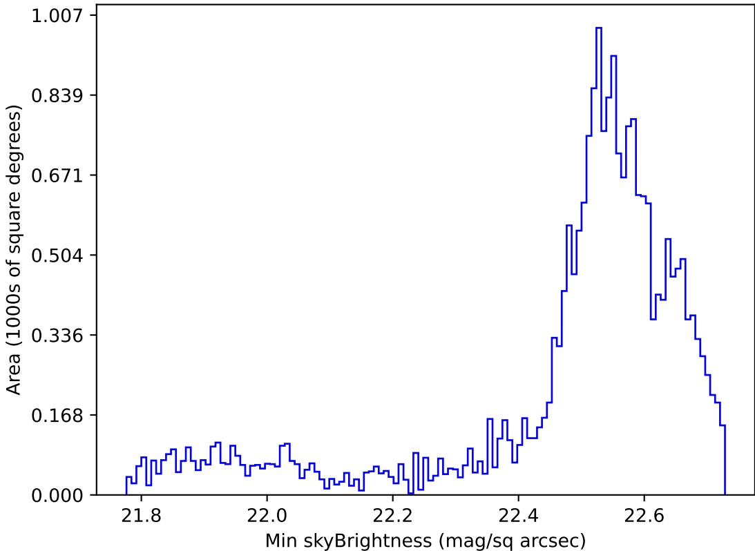
too_elab_r128_d2_griz_v3.4_10yrs Yr 1 u band: Min skyBrightness
