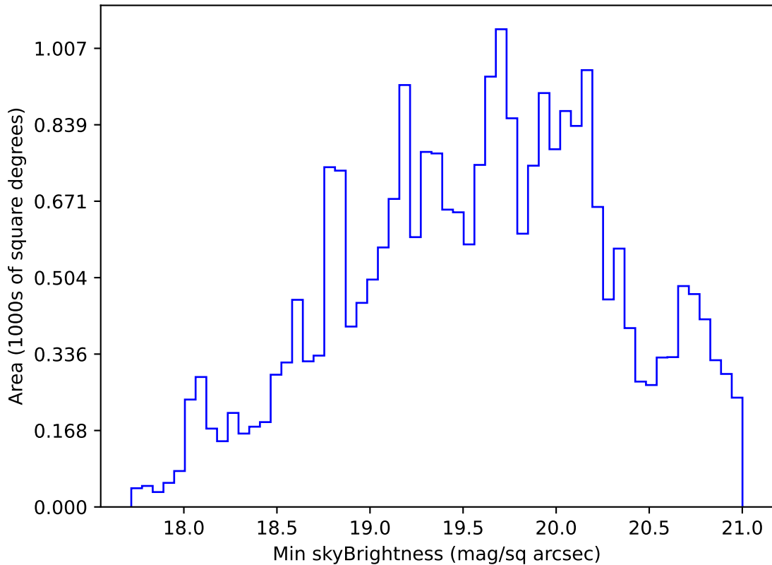
too_elab_r128_d2_griz_v3.4_10yrs Yr 1 r band: Min skyBrightness
