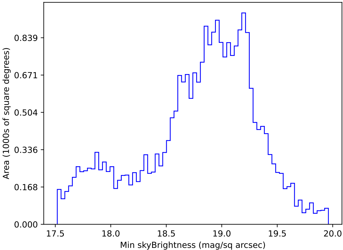
too_elab_r128_d2_griz_v3.4_10yrs Yr 1 i band: Min skyBrightness
