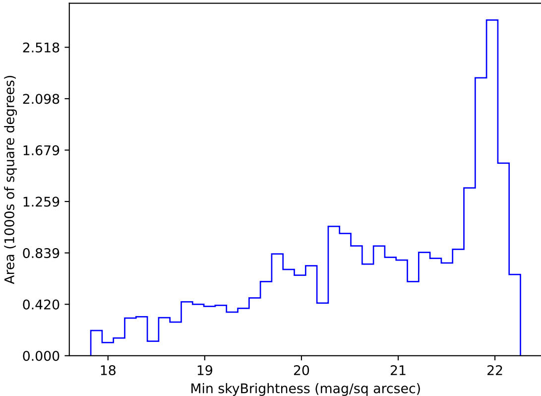
too_elab_r128_d2_griz_v3.4_10yrs Yr 1 g band: Min skyBrightness
