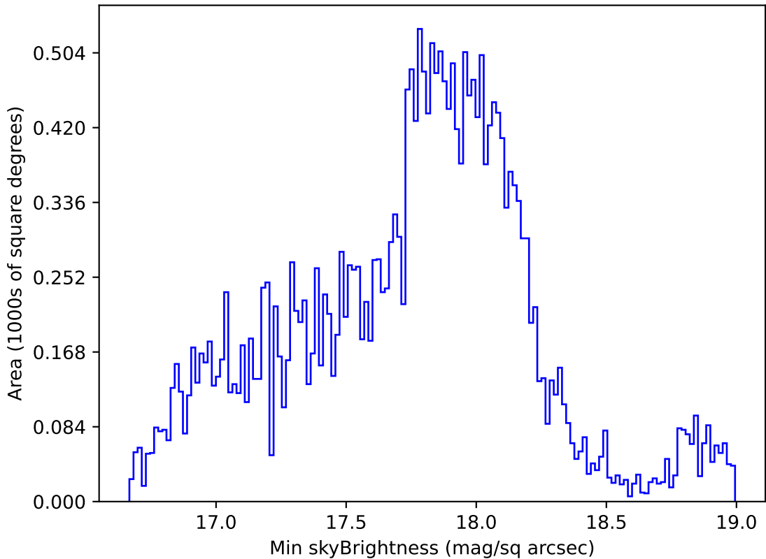
too_elab_r128_d2_griz_v3.4_10yrs Yr 1 all bands: Min skyBrightness
