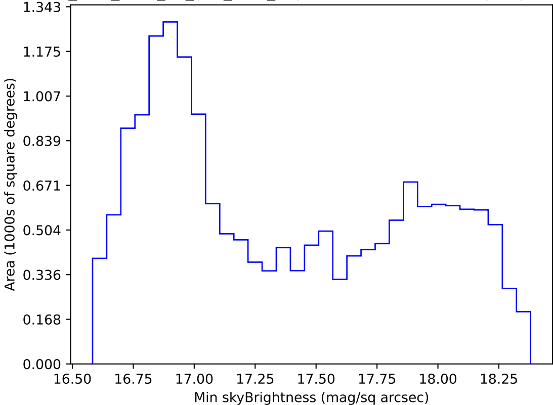
too_elab_r128_d2_griz_v3.4_10yrs WFD z band: Min skyBrightness
