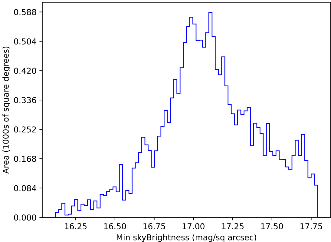
too_elab_r128_d2_griz_v3.4_10yrs WFD y band: Min skyBrightness
