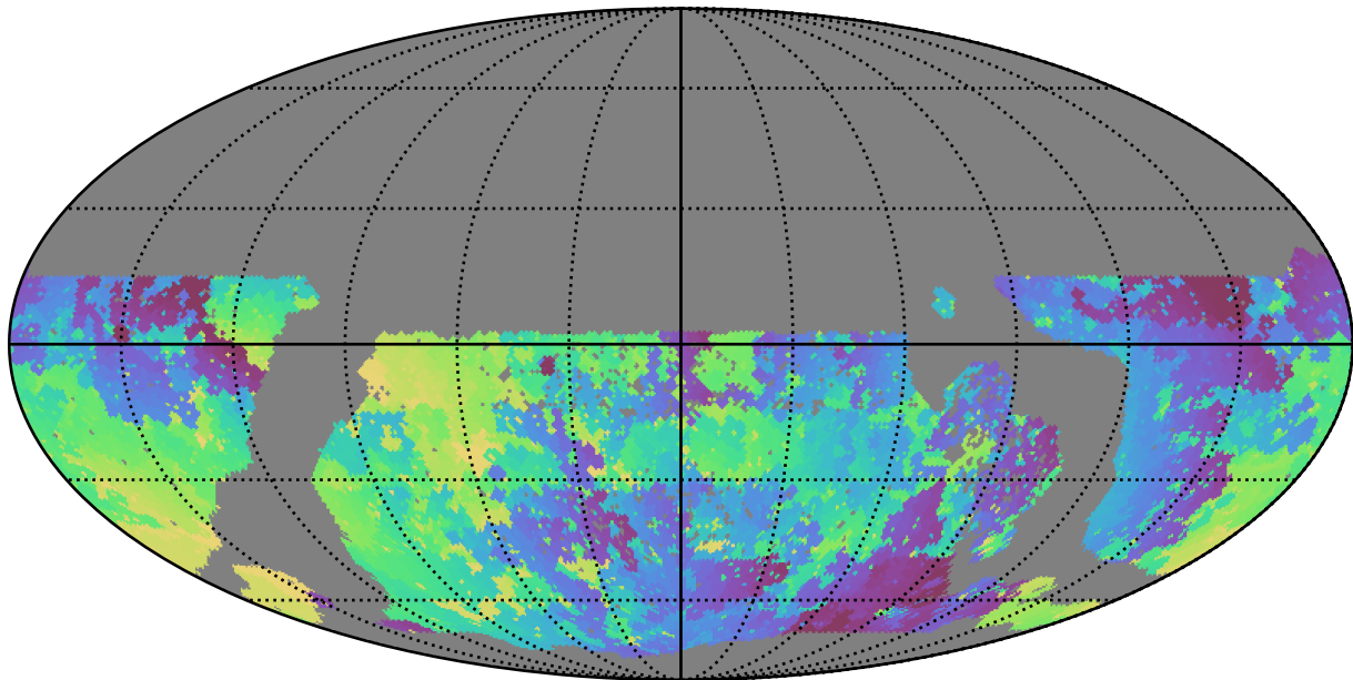
too_elab_r128_d2_griz_v3.4_10yrs WFD u band: Min skyBrightness
