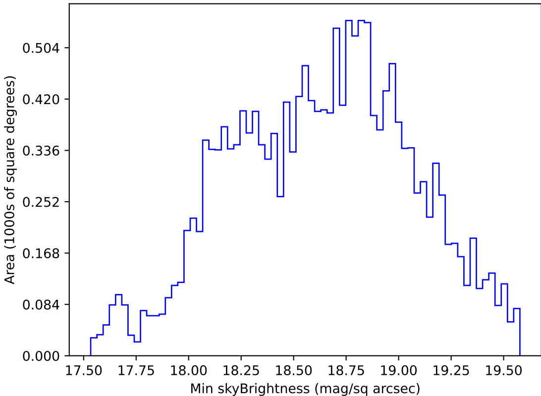
too_elab_r128_d2_griz_v3.4_10yrs WFD r band: Min skyBrightness
