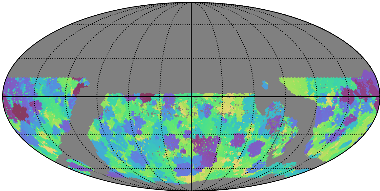
too_elab_r128_d2_griz_v3.4_10yrs WFD g band: Min skyBrightness
