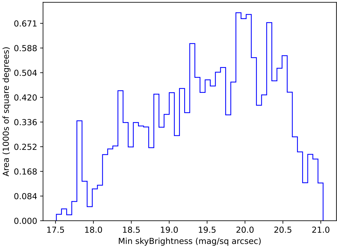
too_elab_r128_d2_griz_v3.4_10yrs WFD g band: Min skyBrightness
