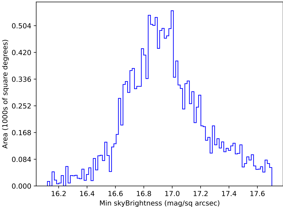
too_elab_r128_d2_griz_v3.4_10yrs WFD all bands: Min skyBrightness
