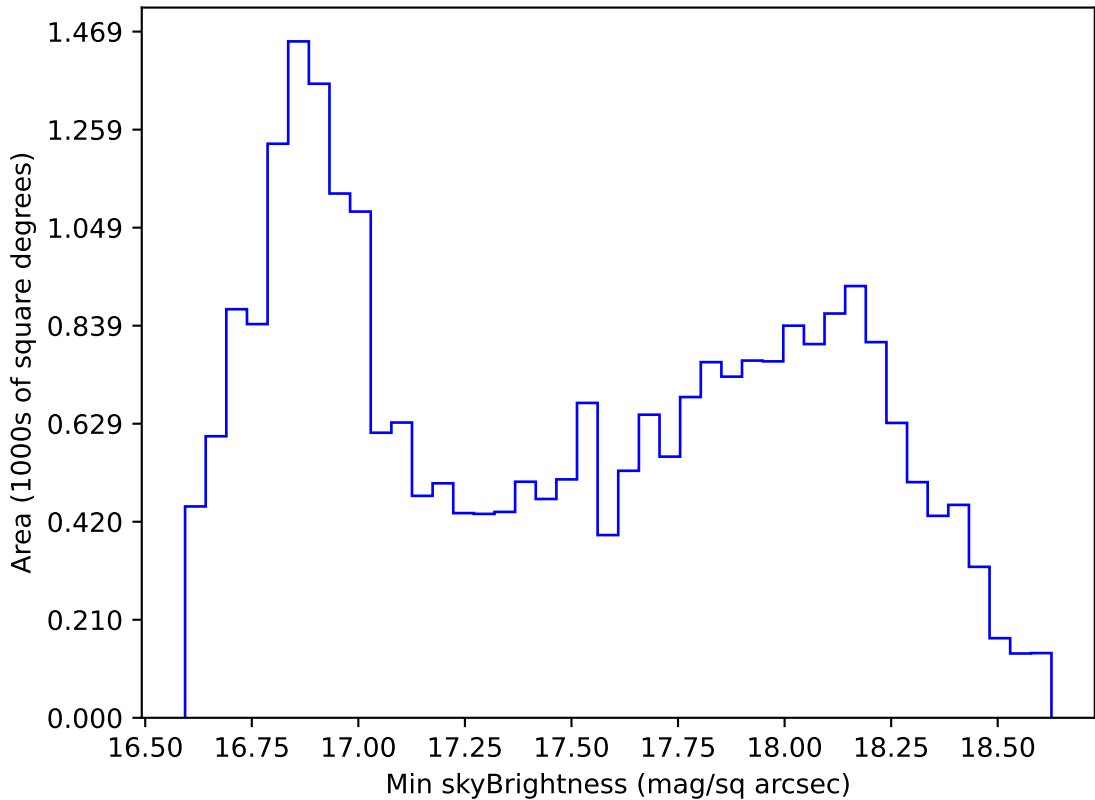
too_elab_r128_d2_griz_v3.4_10yrs All sky z band: Min skyBrightness
