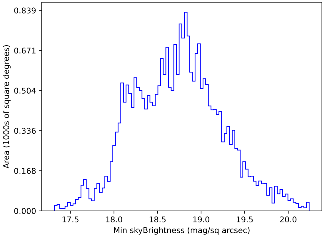
too_elab_r128_d2_griz_v3.4_10yrs All sky r band: Min skyBrightness
