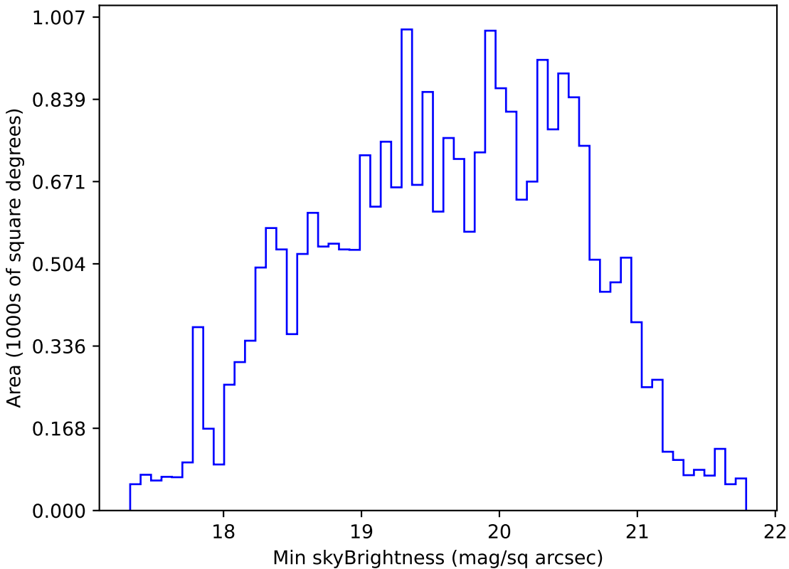
too_elab_r128_d2_griz_v3.4_10yrs All sky g band: Min skyBrightness
