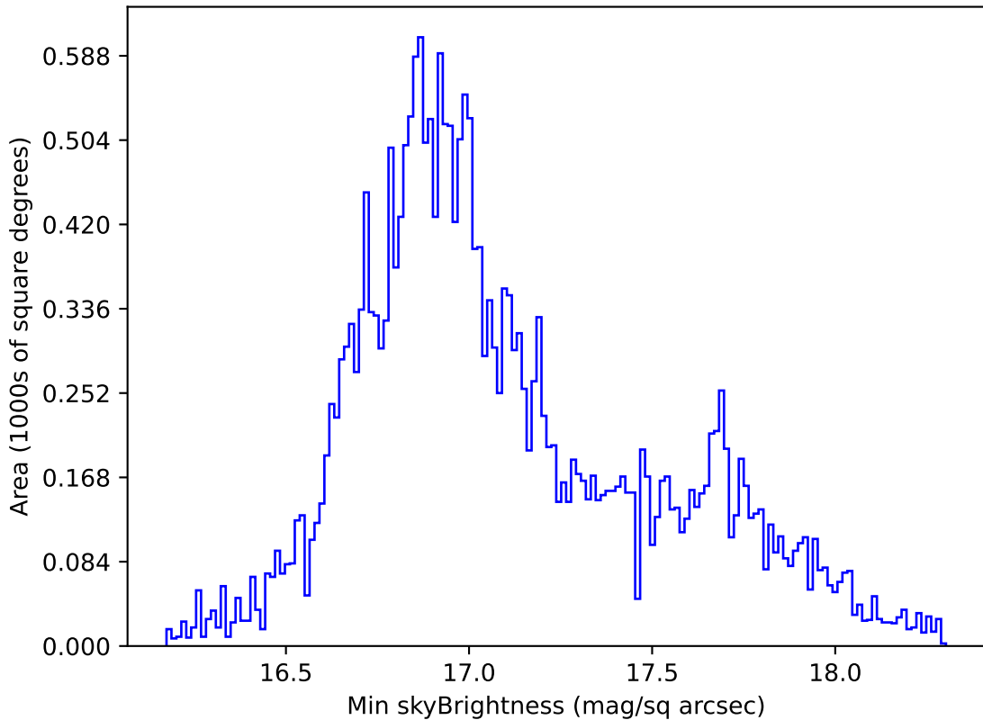
too_elab_r128_d2_griz_v3.4_10yrs All sky all bands: Min skyBrightness
