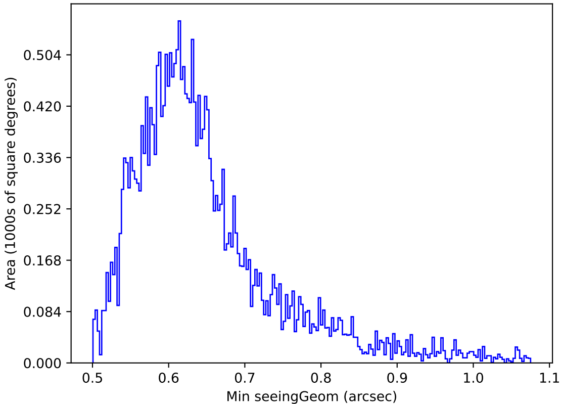
too_elab_r128_d2_griz_v3.4_10yrs Yr 1 z band: Min seeingGeom
