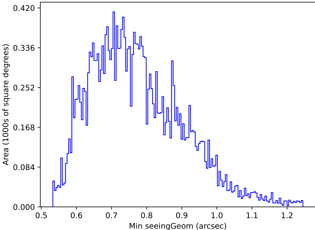
too_elab_r128_d2_griz_v3.4_10yrs Yr 1 u band: Min seeingGeom
