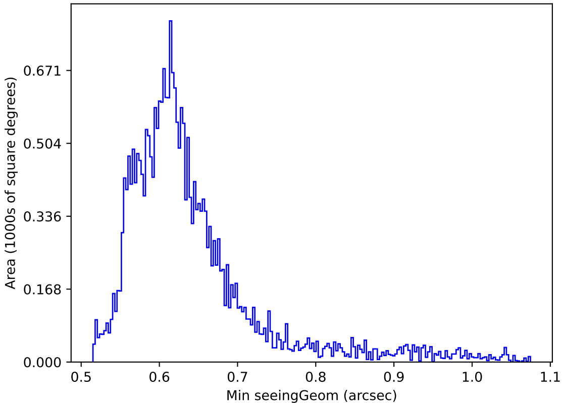
too_elab_r128_d2_griz_v3.4_10yrs Yr 1 r band: Min seeingGeom
