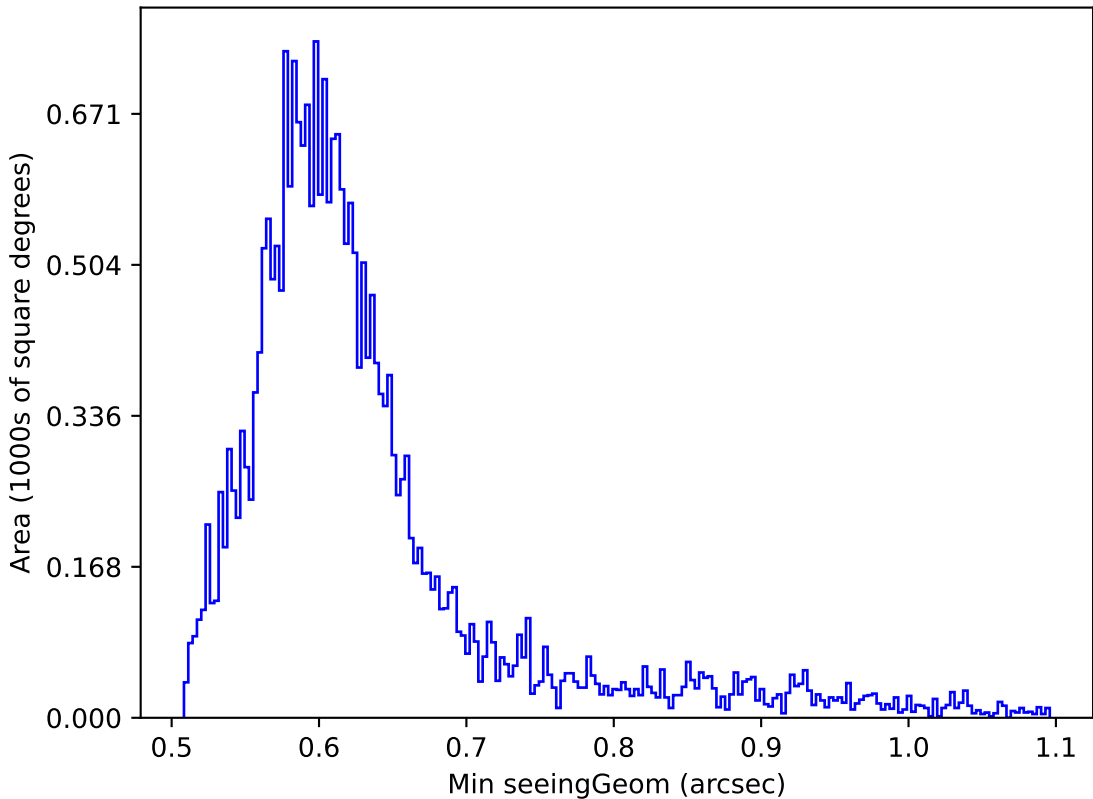
too_elab_r128_d2_griz_v3.4_10yrs Yr 1 i band: Min seeingGeom
