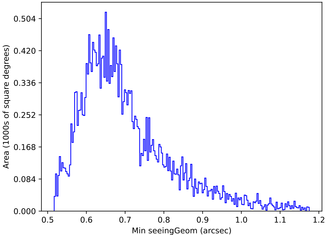
too_elab_r128_d2_griz_v3.4_10yrs Yr 1 g band: Min seeingGeom
