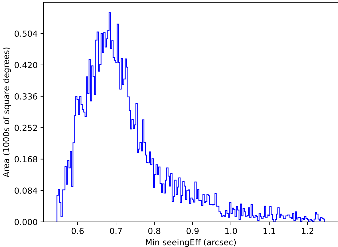
too_elab_r128_d2_griz_v3.4_10yrs Yr 1 z band: Min seeingEff
