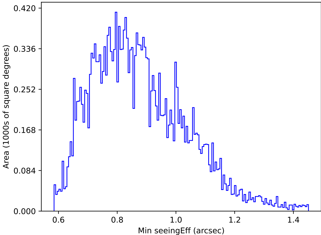
too_elab_r128_d2_griz_v3.4_10yrs Yr 1 u band: Min seeingEff
