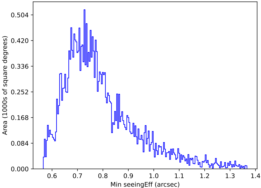
too_elab_r128_d2_griz_v3.4_10yrs Yr 1 g band: Min seeingEff
