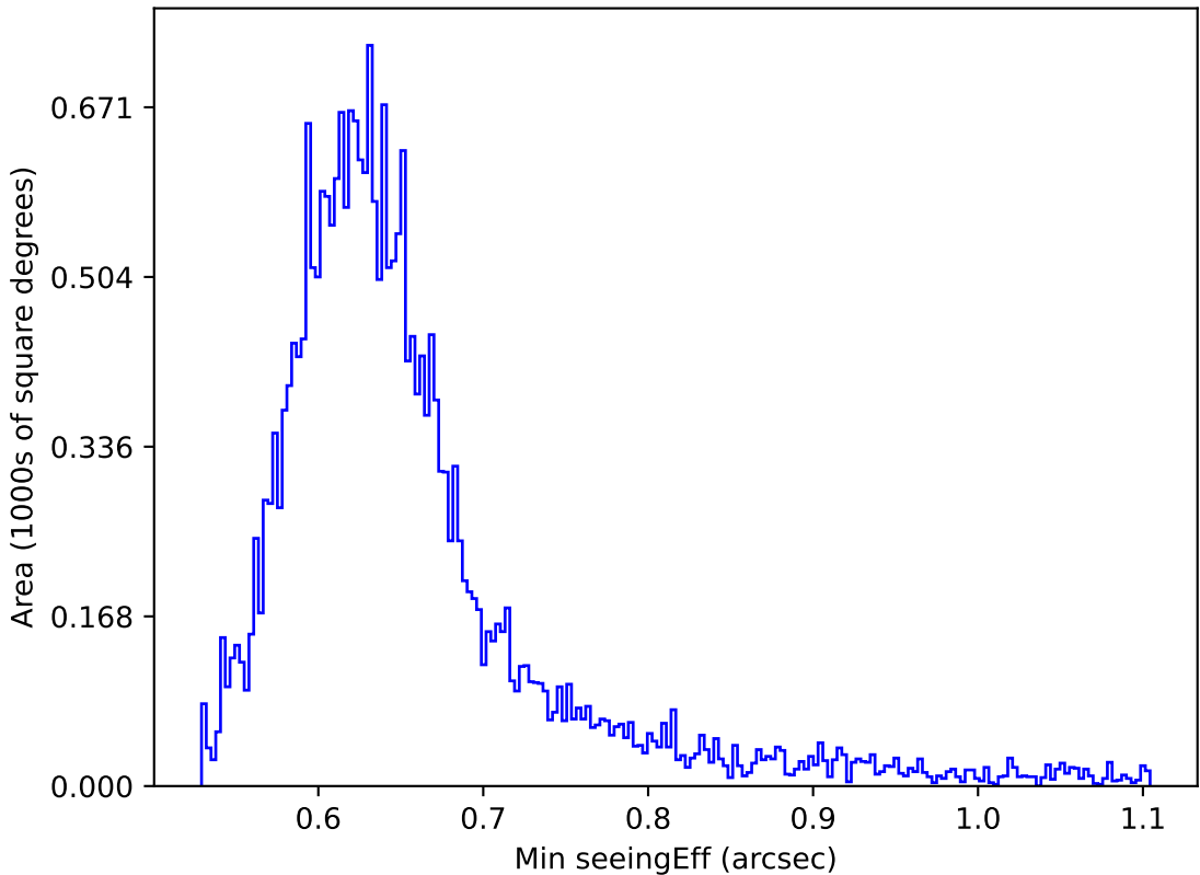
too_elab_r128_d2_griz_v3.4_10yrs Yr 1 all bands: Min seeingEff
