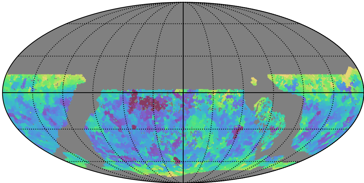
too_elab_r128_d2_griz_v3.4_10yrs WFD y band: Min seeingEff
